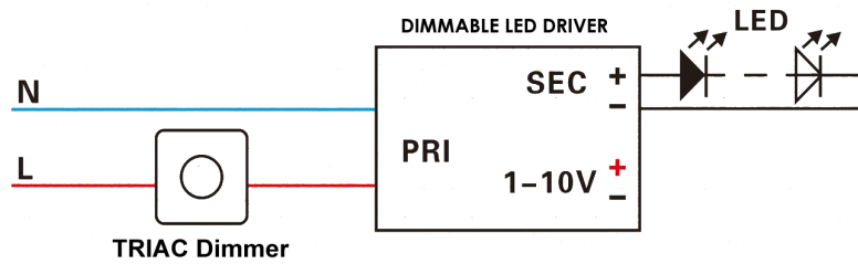
TRIAC (SRC) Dimmable Wiring Diagram
